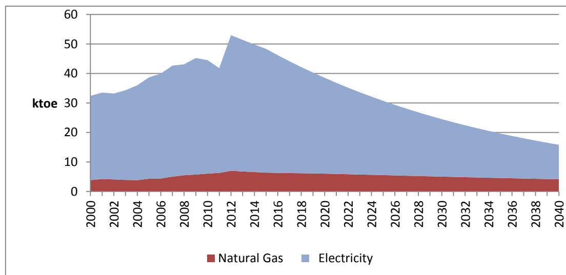
Figure 28: Commercial Sector Energy Use in Barbados under the Sustainable Energy Framework
