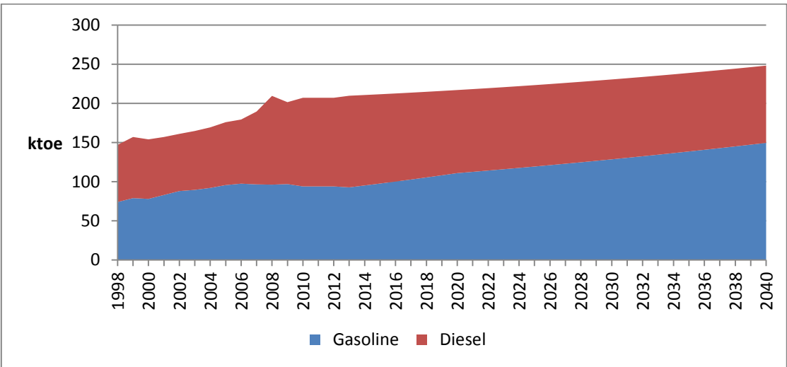
Figure 27: Transport Sector Fuel Use under the Sustainable Energy Framework
