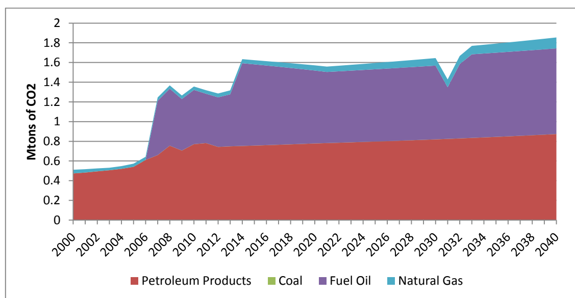
Figure 16: CO 2 Emissions from Fuel Combustion in Barbados under BAU
