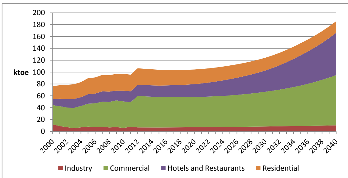
Figure 18: Final Energy Use by Sector under the National Strategic Plan
