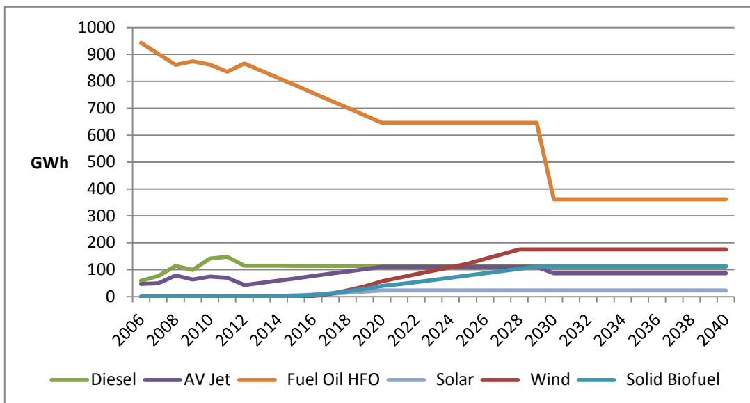
Figure 31: Electricity Production by Fuel Type and Energy Source in Barbados under the Sustainable Energy Framework
