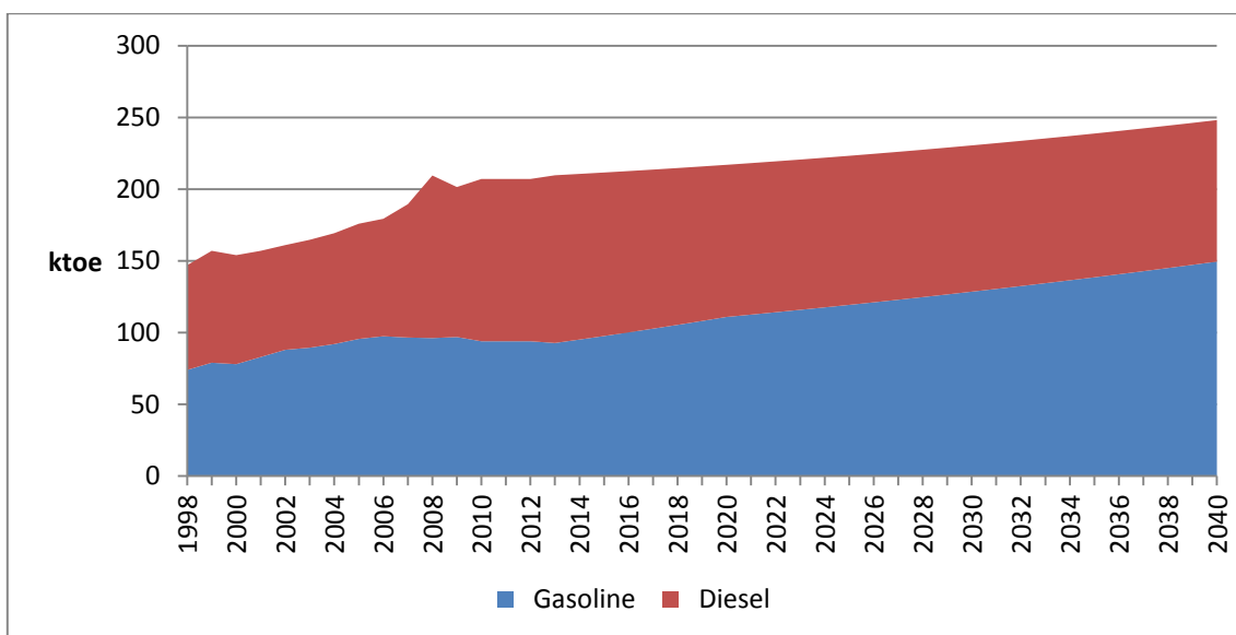
Figure 10: Transport Sector Fuel Use In Barbados given BAU Assumptions
